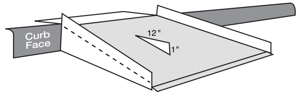
BoardWalk Ramp has a maximum slope of 8%, or 1:12 ratio.
