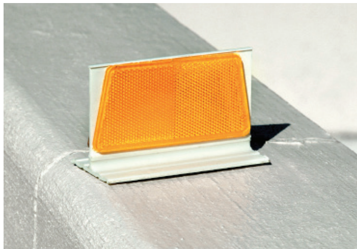
BAM Delineator, clear lens, on side, Quik-Mark Object Marker, on top.
